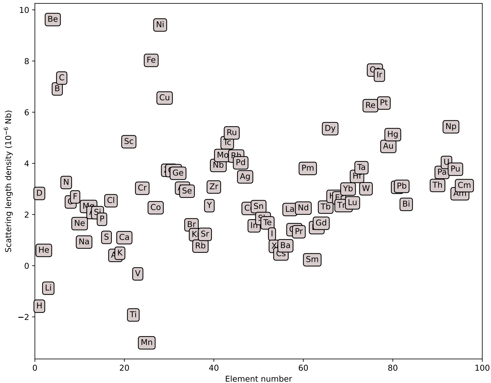
Neutron SLD for elements in natural abundance
